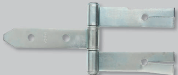
Double rod gate hinge for anchoring and screwing
